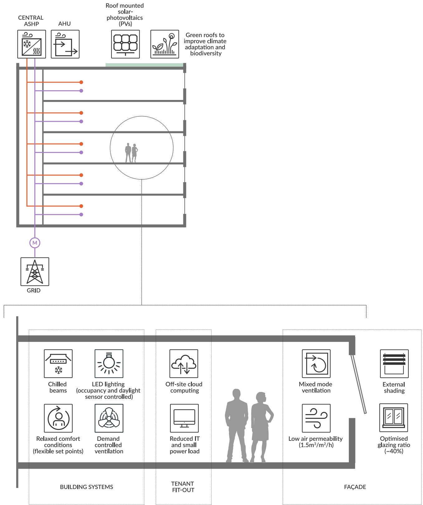
Figure 11: Design schematic for net zero offices (including additional features not addressed within this study)
