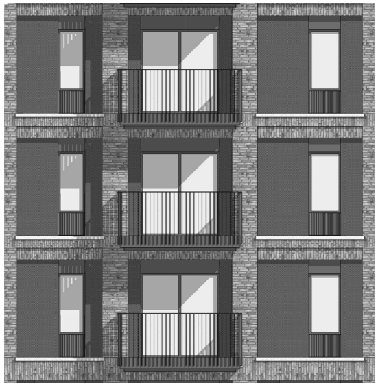
Figure 16: The original design included juliette balconies to most bedrooms (left), however this has been removed for the stretch design to reduce glazing areas (right)
