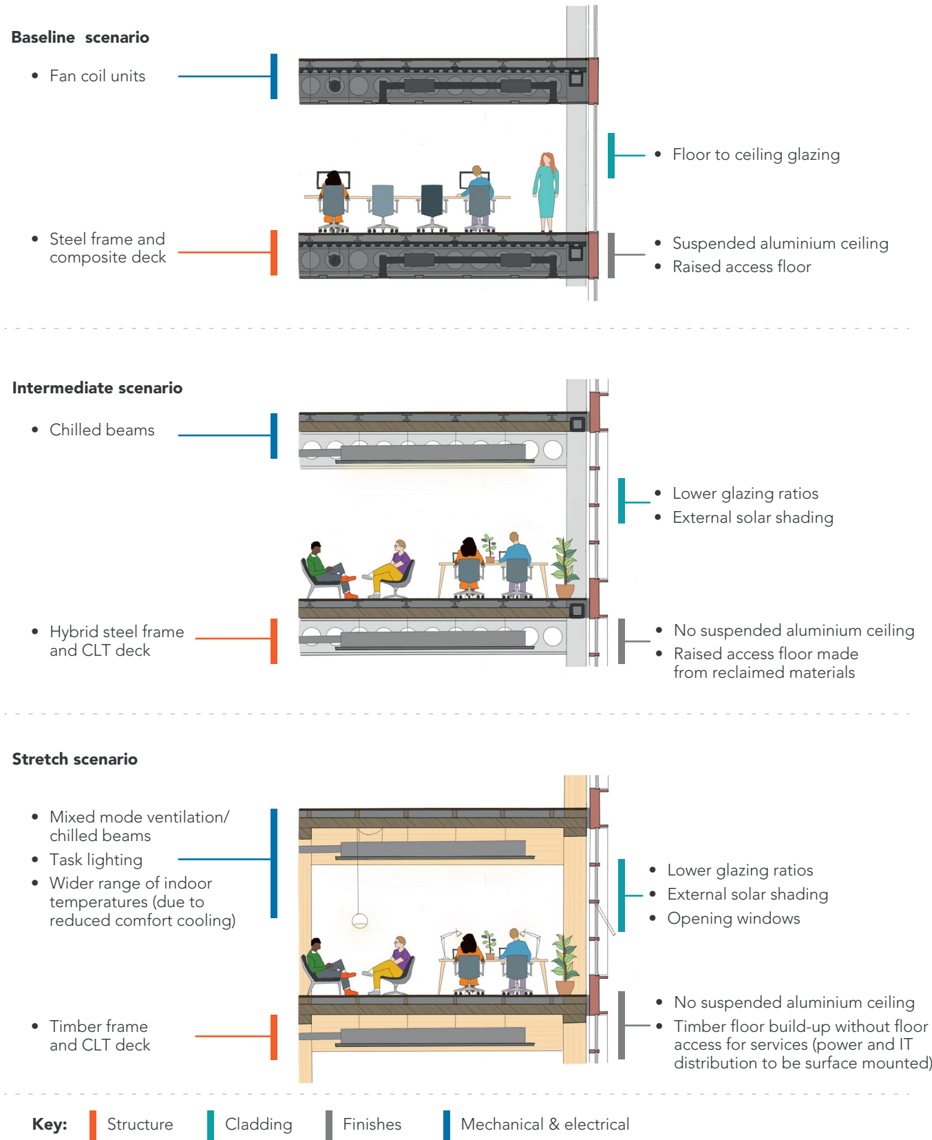
Figure 10: Illustration of the upgraded facade and internal fitout spaces
