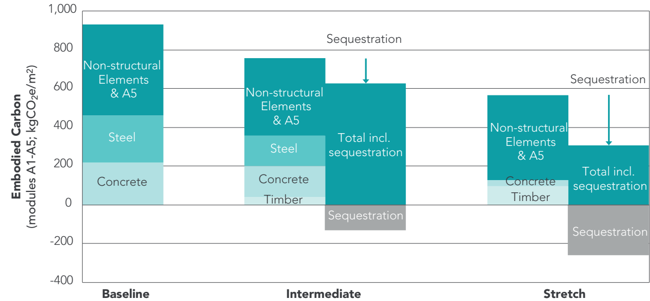
Figure 9: Chart showing the reduction in upfront carbon across all three scenarios based on changes to the structural design
