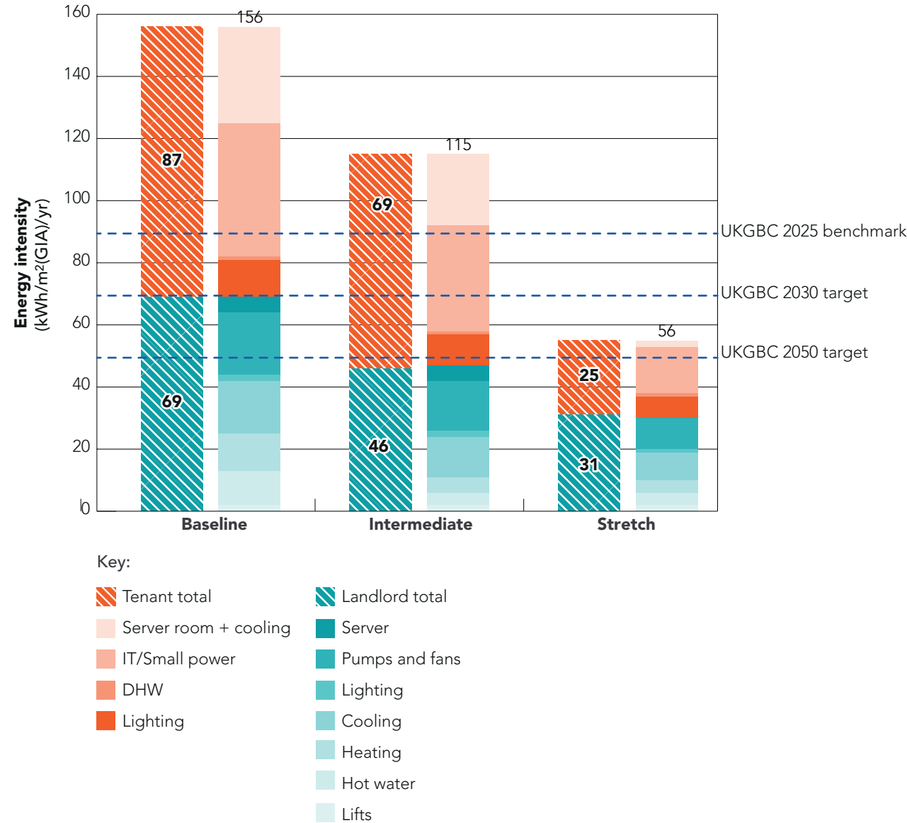
Figure 12: Whole building energy use across three scenarios
